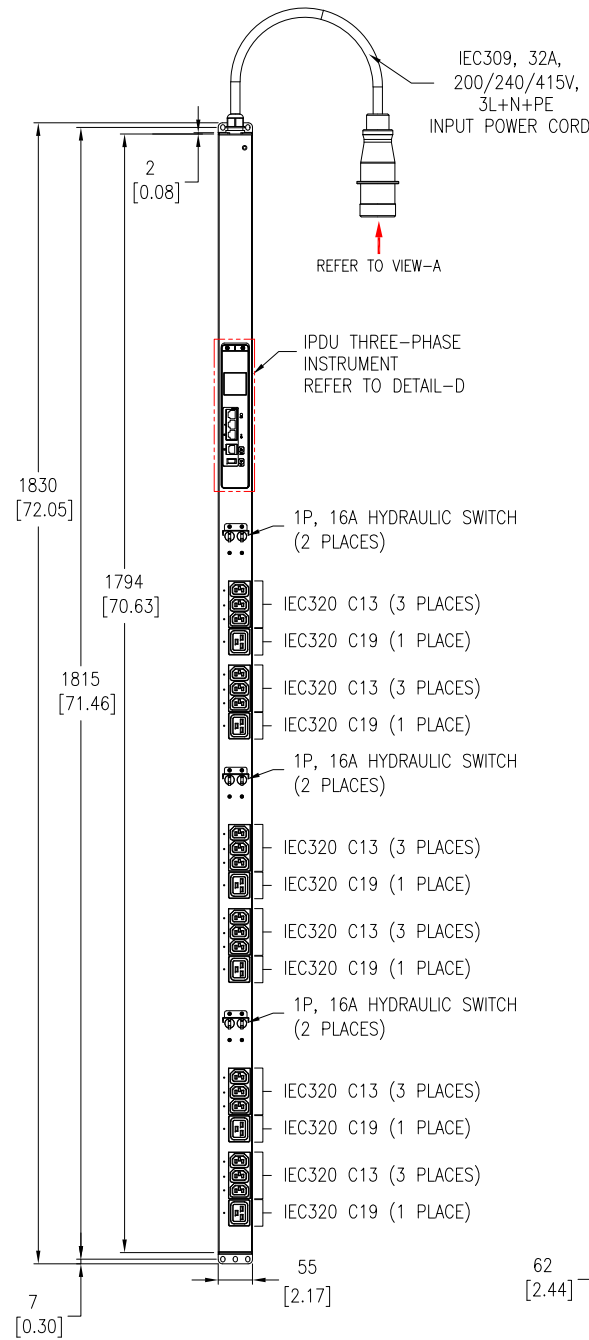
FRONT VIEW
