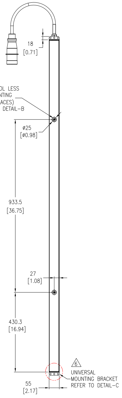
REAR VIEW
